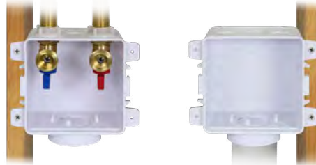
Dual Boxes Inbetween Studs
